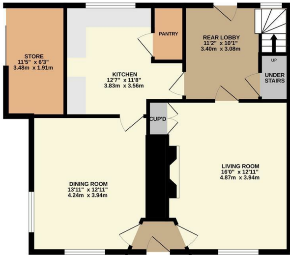
GROUND FLOOR 717 sq.ft. (66.6 sq.m.) approx.
